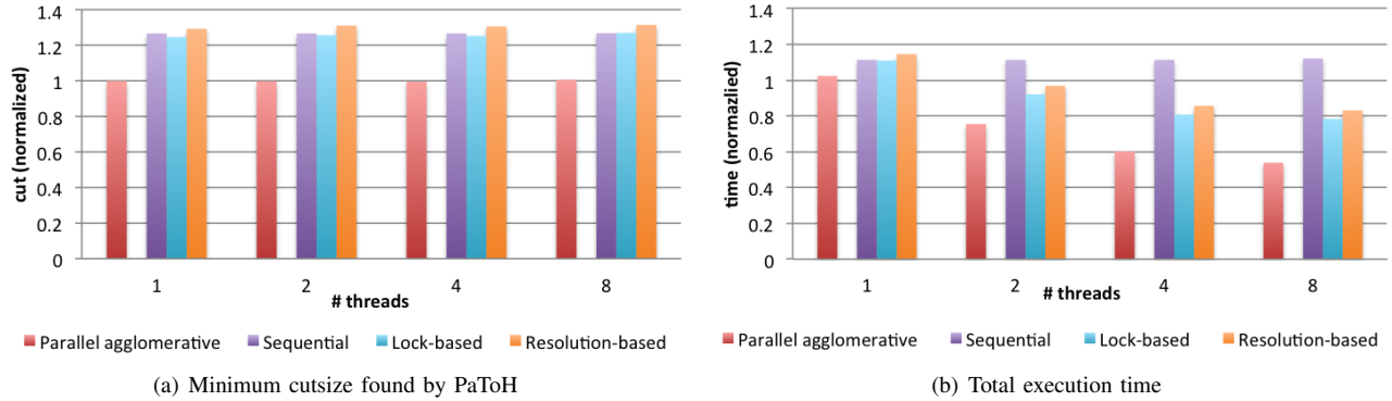
Figure 6. The minimum cut and execution time of PaToH when equipped with the clustering algorithms in this paper. The numbers are normalized with respect to that of agglomerative clustering algorithm.
