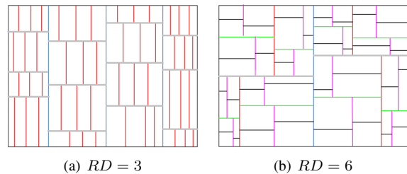
Figure 2. Partitioning into 64 parts using MJ with different recursion depths. Cutlines in the same level of recursion share the same color.
