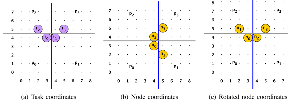
Figure 4. An example showing the benefit of rotating the node orientation. Assuming communication is required between only tasks 0 and 2, the unrotated mapping (4(b)) has average hop count of 1 and 1 in the x and y directions, respectively. In the rotated node-partition (4(c)), partitioning is performed in the y dimension first, and then in the x dimension. The mapping obtained after rotation has average hop count of 1 and 0 in x and y .
