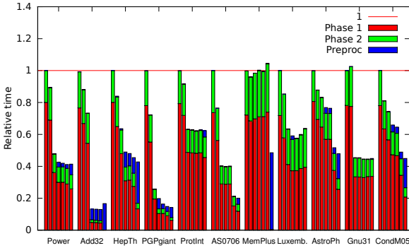
(a) Normalized execution times for small graphs
